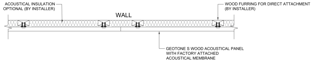
GEOTONE DIRECT ATTACHMENT - PLAN VIEW
